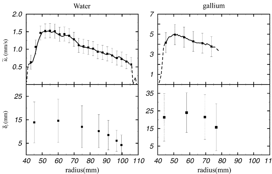
Fig. 6. Mean properties for the flow extracted from patterns 3 and 4. Broken line in gallium plots of this figure and Fig. 7 highlights the region where the signal is saturated by multiple echoes due to the impedance contrast between copper and liquid gallium.
