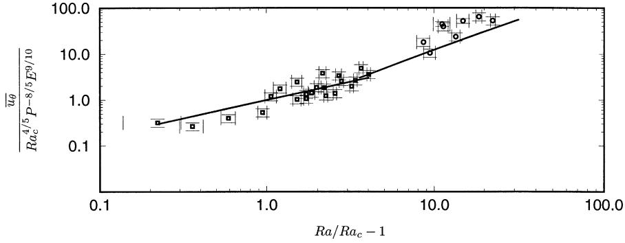
Fig. 12. Reduced zonal flow velocity. Solid line is y \sim ((Nu - 1)(Ra/Ra_c - 1))^{4/5} in water and y \sim (Ra/Ra_c - 1)^{4/5} in gallium. Scaling prefactor is 1.
