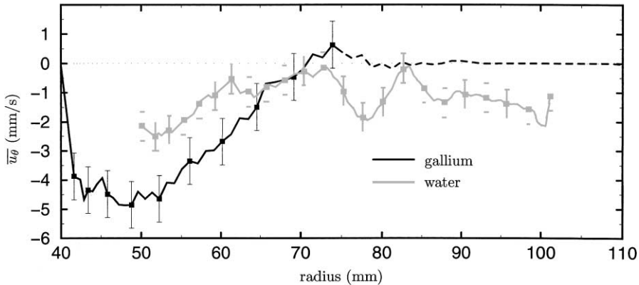
Fig. 7. Mean zonal flow \bar{u}_\theta in water (experiment 5: E = 4.8 \times 10^{-6} , Ra = 31Ra_c ), and gallium (experiment 6: E = 1.5 \times 10^{-6} , Ra = 3.2Ra_c ).
