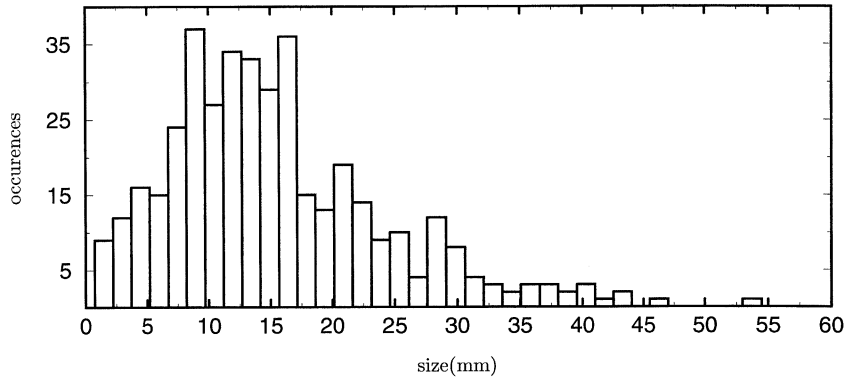
Fig. 14. Histogram of the distribution of radial cell sizes in the convective flow, measured at radius 60 mm in water, for experiment of Fig. 4c (Ekman number is 4.8 \times 10^{-6} , Rayleigh number is 26.6 times critical).
