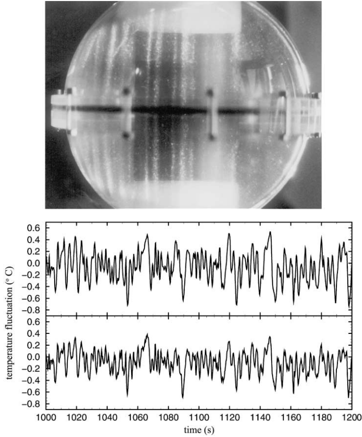
Fig. 3. Top: shear structures visualized in water using Kalliroscope flakes, in a plane containing the rotation axis, close to the inner cylinder. Ekman number is E = 9.7 \times 10^{-6} , Rayleigh number is 4.2 times critical. Bottom: vertical correlations between two thermocouple probes located 5 cm away on the inner cylinder, done in gallium. Ekman number is E = 7.3 \times 10^{-7} , Rayleigh number is five times critical.
