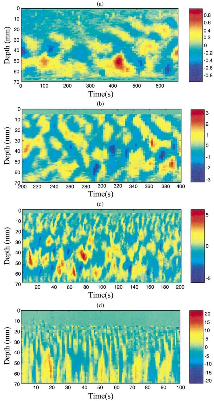
Fig. 4. Time-depth radial velocity patterns. Velocities are expressed in mm/s. (a) Performed in water, with Ra/Ra_c = 4.2 , E = 9.7 \times 10^{-6} . (b) Performed in water, with Ra/Ra_c = 22.2 , E = 9.7 \times 10^{-6} . (c) Performed in water, with Ra/Ra_c = 26.6 , E = 4.8 \times 10^{-6} . (d) Performed in liquid gallium, with Ra/Ra_c = 3.2 , E = 1.5 \times 10^{-6} .
