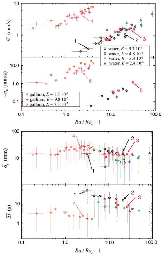
Fig. 8. Scalar data extracted for scaling. Arrows 1–4 denote data points corresponding to shown velocity patterns (Fig. 4). Arrows 5 and 6 correspond to zonal flows shown on Fig. 7.
