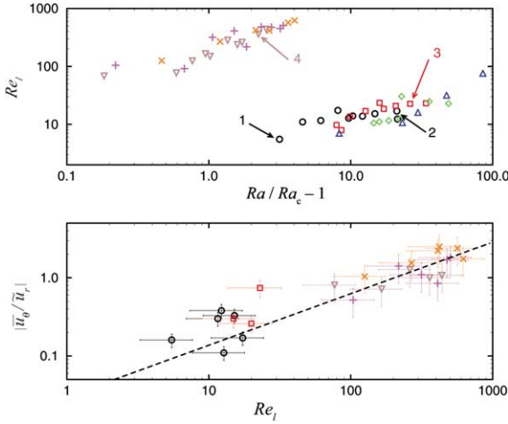
Fig. 9. Scalar data (continued).
