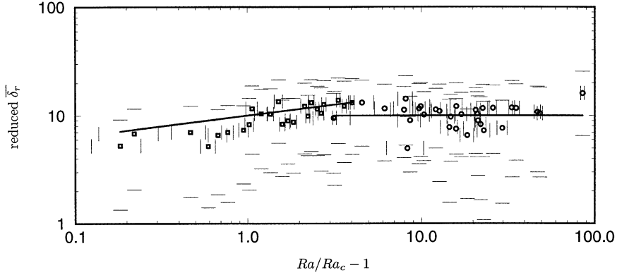
Fig. 11. Reduced cell size for gallium (squares) and water (circles) experiments. The viscous scaling is tested for water experiments, the reduced cell size is, therefore, \overline{\delta_r}/E^{1/3} . The inertial scaling is tested for gallium experiments, the reduced cell size is, therefore, \overline{\delta_r}/(Ra_Q^{1/5} P^{-2/5} E^{3/5}) . Solid line in gallium corresponds to dependence y \sim (Ra/Ra_c - 1)^{1/5} . Solid line in water is y \sim 1 . Both prefactors are 10.
