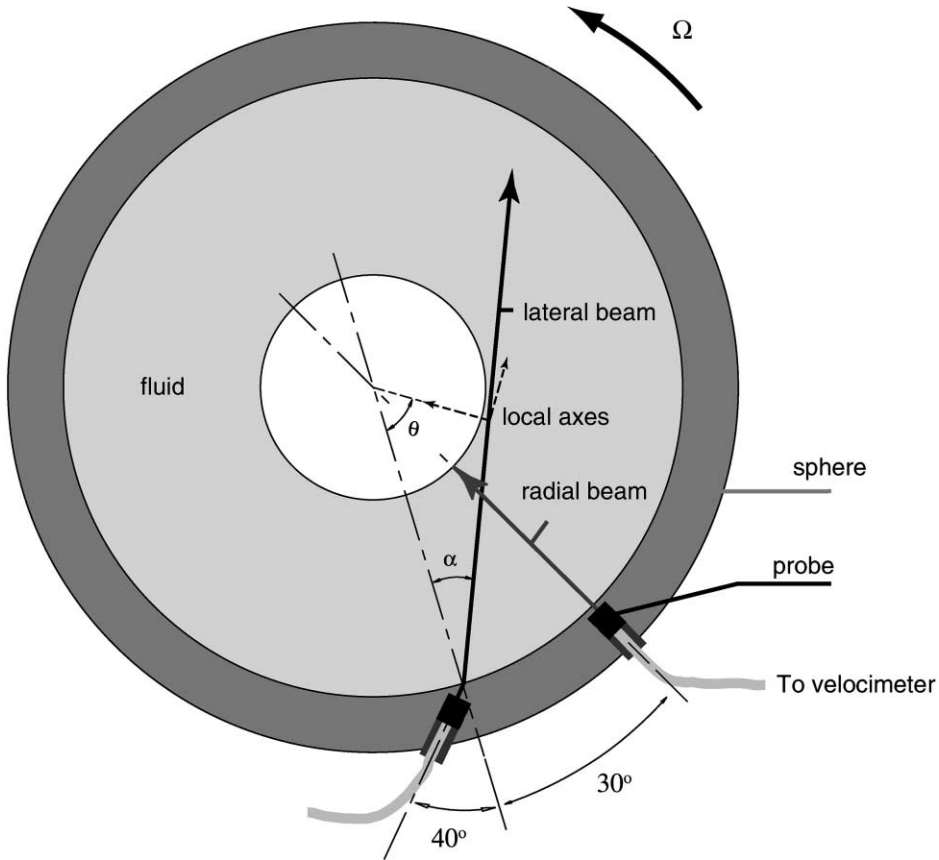
Fig. 2. Top view of the equatorial plane, with locations of transducers.
