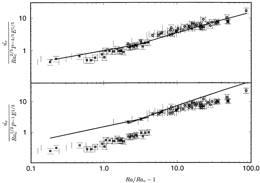
Fig. 10. Reduced radial velocity for gallium (squares) and water (circles) experiments. Top: test of the inertial balance. Solid line in water corresponds to theoretical dependence y \sim ((Nu-1)(Ra/Ra_c-1))^{2/5} with Nu \sim (Ra/Ra_c)^{1/2} . Solid line in gallium corresponds to dependence y \sim (Ra/Ra_c - 1)^{2/5} . Scaling prefactor is 1. Bottom: test of the viscous balance. Solid line in water is y \sim ((Nu - 1)(Ra/Ra_c - 1))^{1/2} , and in gallium y \sim (Ra/Ra_c - 1)^{1/2} . Prefactor is 1.5.
