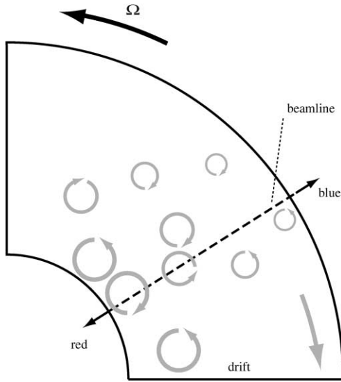
Fig. 5. Explanation sketch for time–depth velocity maps.
