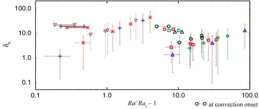
Fig. 13. Lateral size of vortices at radius r_{\max} , near the inner cylinder.
