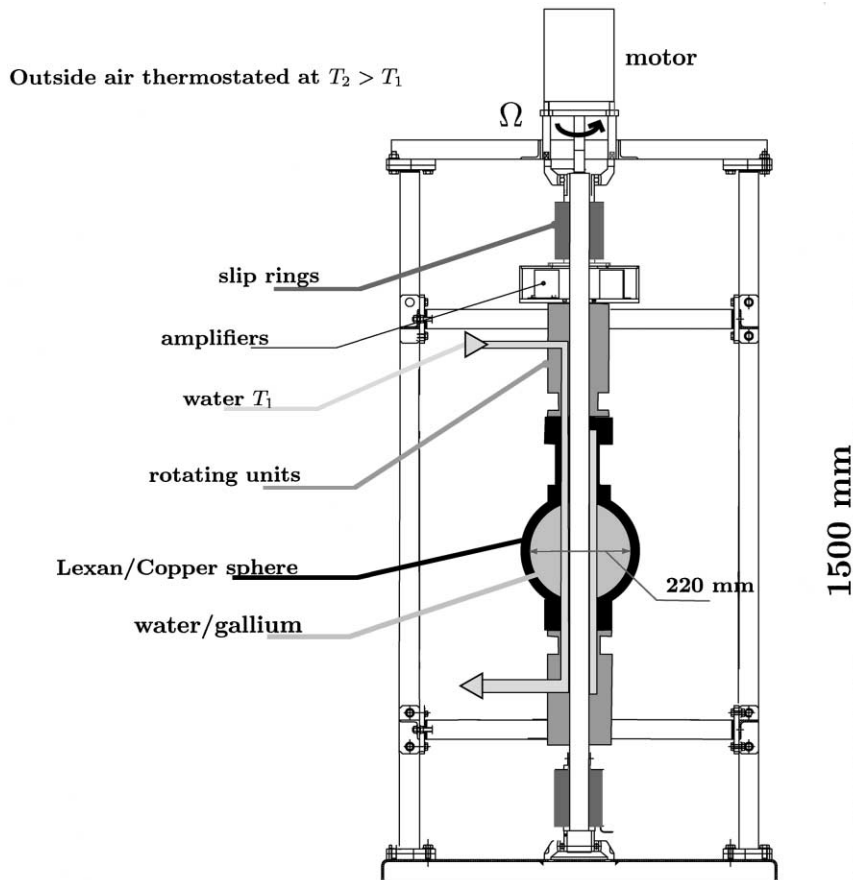
Fig. 1. Sketch of the convection device.
